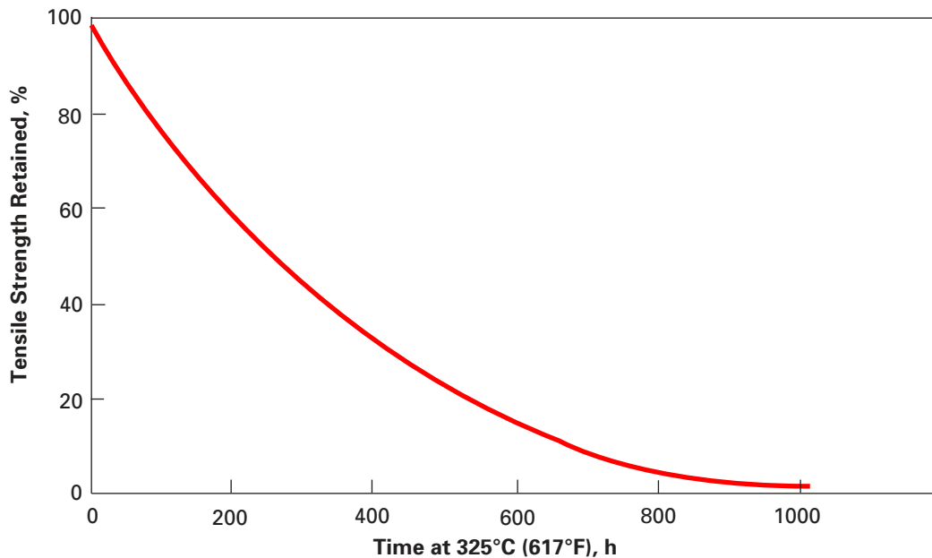
Figure 6. Tensile Strength vs. Aging in Air at 325°C (617°F), Type HN Film, 25 μm (1 mil)
